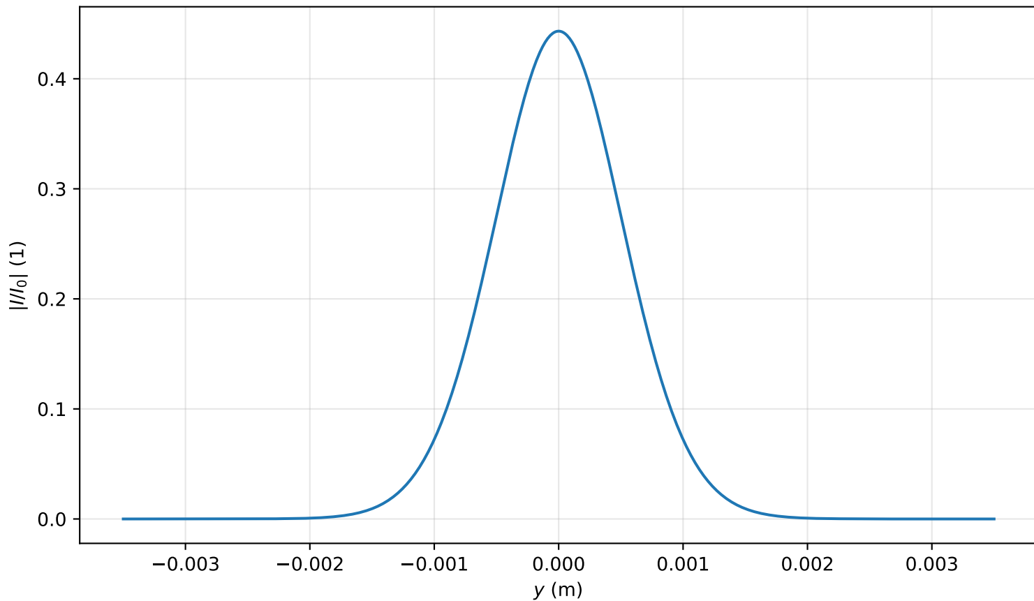
Intensity profile I(x=0, y, z=2.627)/I_0 , P_{in}=0.2P_{cr} , artificial time
